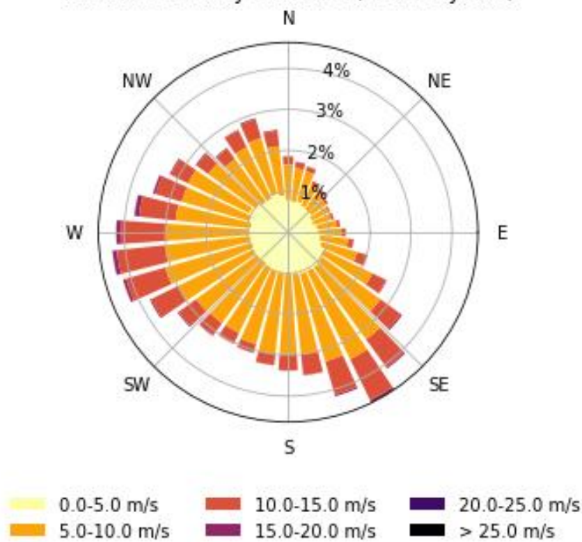
Figure 9.4 – 20-year projected wind speeds and directions covering the period 01/01/2000 – 05/08/2020
