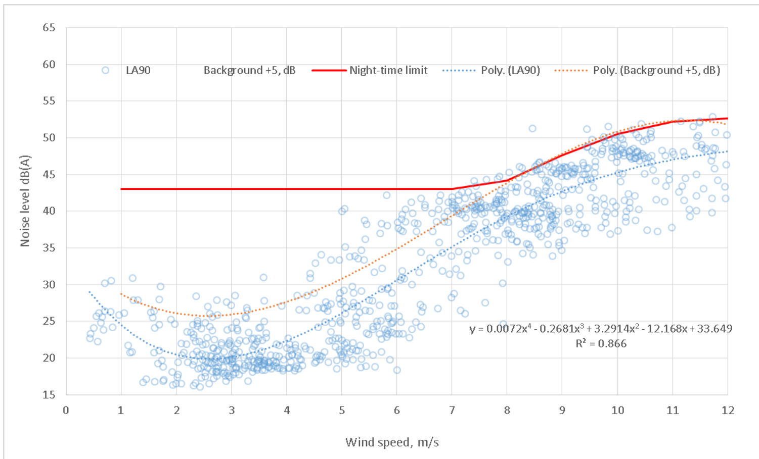
Chart 9.6 - Noise Limit Derivation at NMP2, Night-time Period
