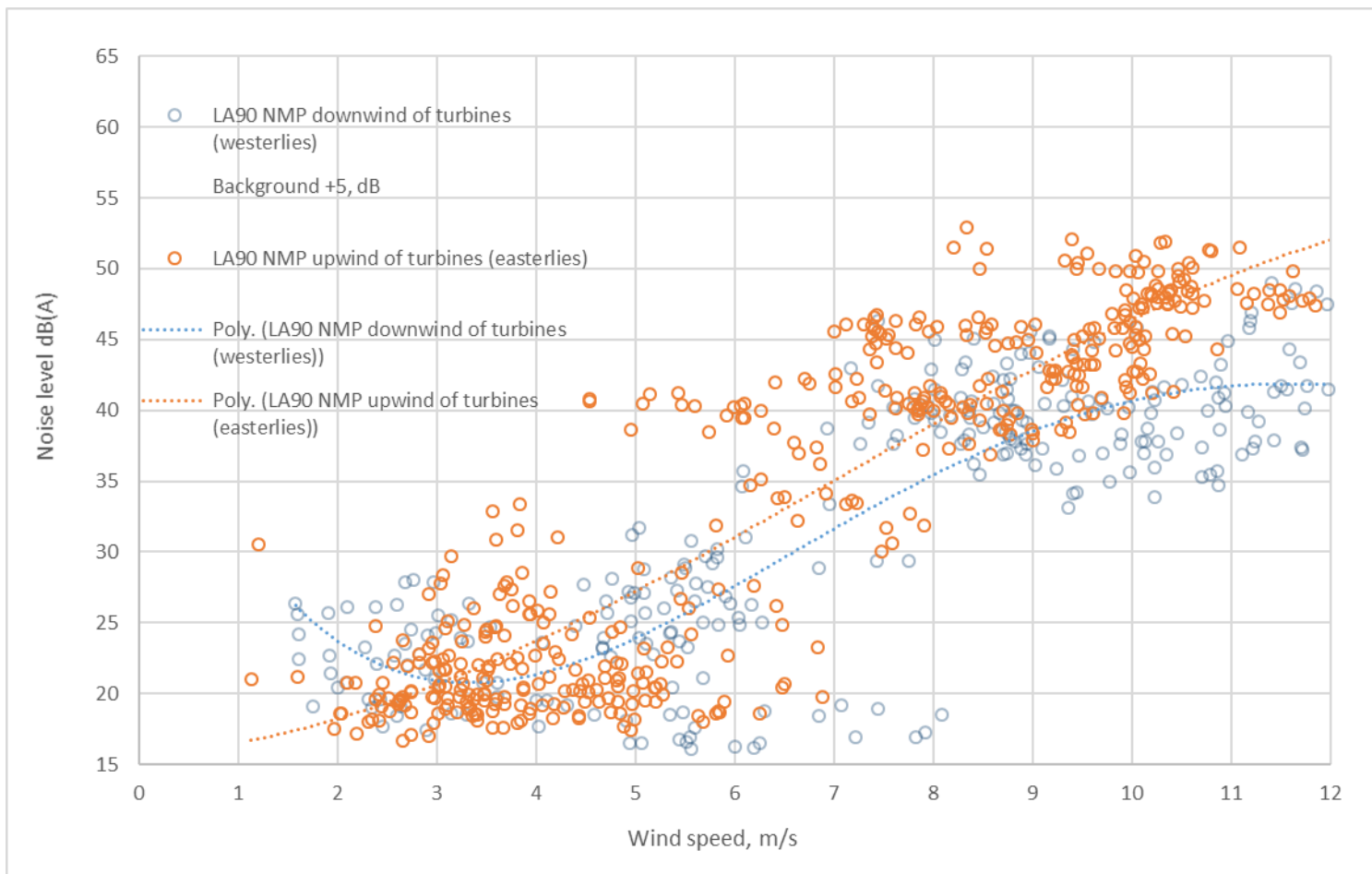
Chart 9.8 – Results of directional filtering of measured data at NMP2, night-time period
