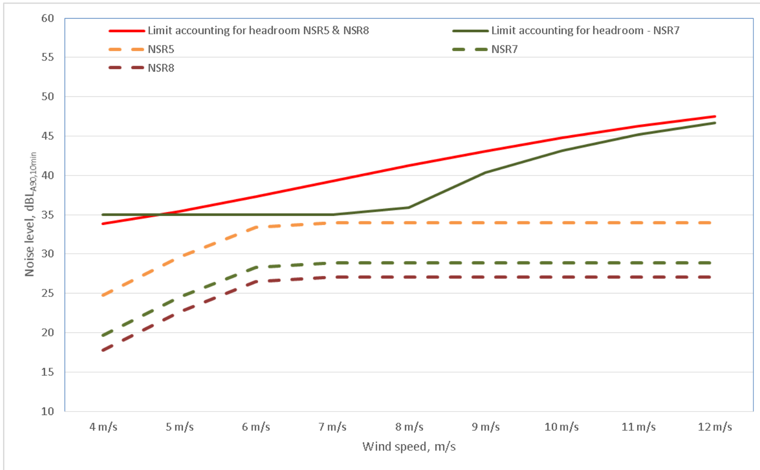
Chart 9.12 – Evaluation of predicted noise levels against noise limits – Cumulative NSRs at which NMP1 derived noise limits apply, night-time period
