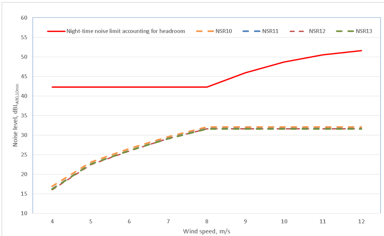
Chart 9.14 – Evaluation of predicted noise levels against noise limits – Proposed Development only, NSRs at which NMP2 derived noise limits apply, night-time period
