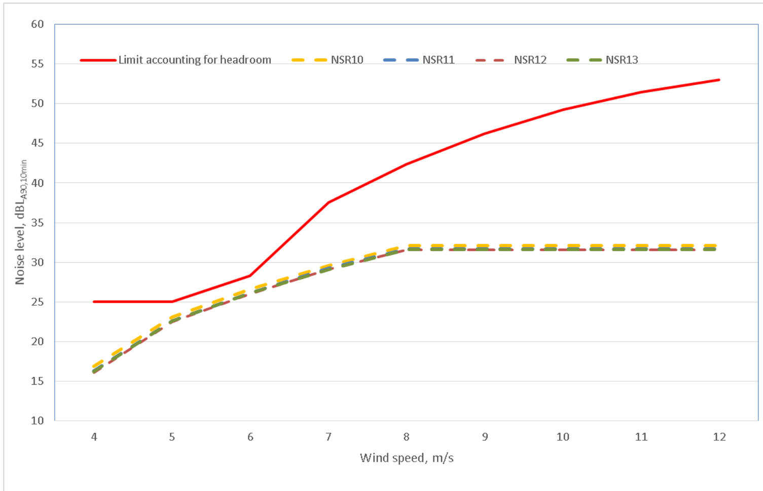
Chart 9.14 – Evaluation of predicted noise levels against noise limits – Proposed Development only, NSRs at which NMP2 derived noise limits apply, night-time period
