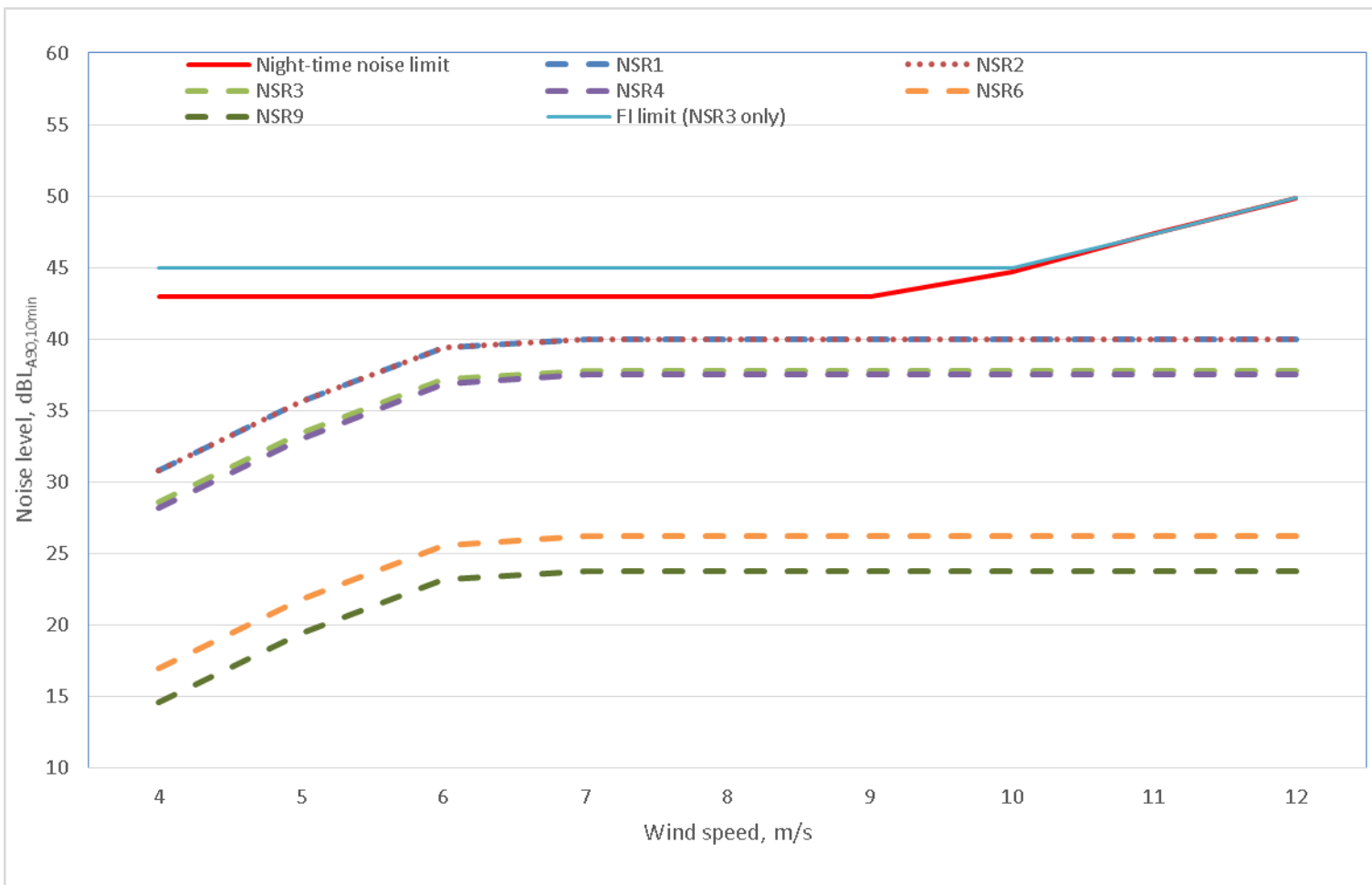
Chart 9.10 – Evaluation of predicted noise levels against noise limits – non-cumulative NSRs at which NMP1 derived noise limits apply, night-time period
